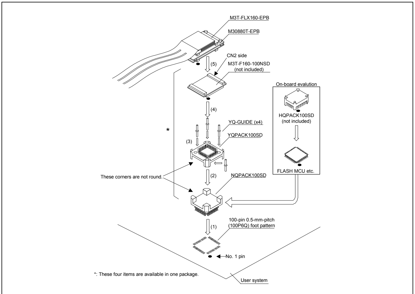
Figure 2.14 Connecting to a 100-pin 0.5-mm-pitch foot pattern (3/3)
